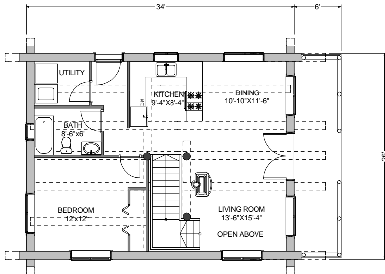
MAIN FLOOR PLAN 884 SQ. FT.
