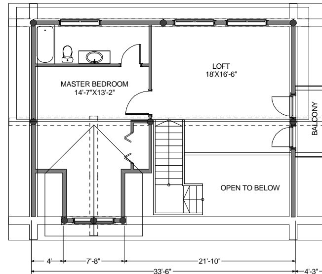
LOFT PLAN 640 SQ. FT.
